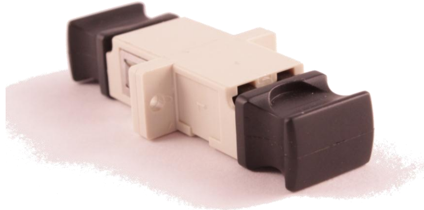
P/N : 48MMTLCD LC/LC UPC duplex beige adapter MM with flange Suitable for OM1/OM2/OM3/OM4
